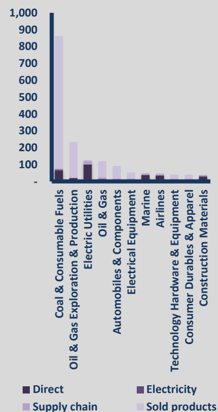
FIG 4.2: GHG EMISSIONS BY Scope FOR A SAMPLE OF SECTORS (SOURCE: ADEME 2012)
