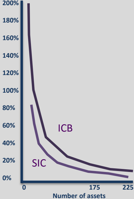
FIG 4.6: SHARE OF UNCERTAINTY OF PORTFOLIO CARBON FOOTPRINT BY # OF ASSETS/SECTOR CLASSIFICATION (SOURCE: BOFAML 2011)
