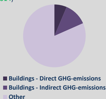
FIG 2.6: SHARE OF BUILDINGS IN DIRECT AND INDIRECT GHG EMISSIONS, 2010 (SOURCE: IPCC 2014)
